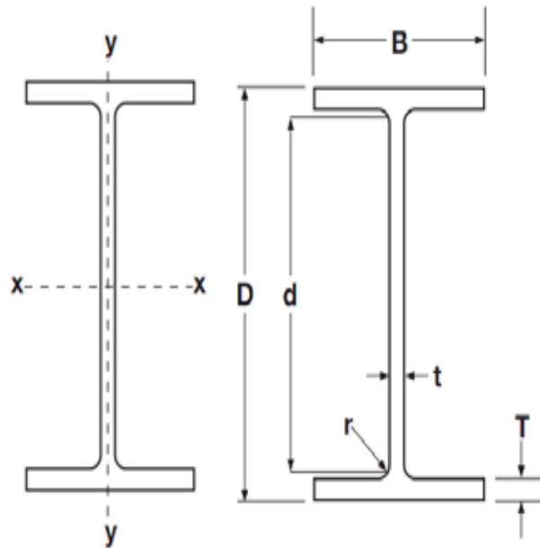
Universal Column Section
