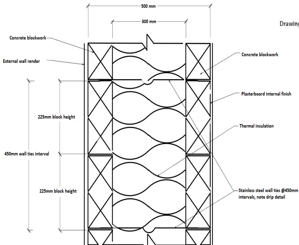
External wall section sketch
