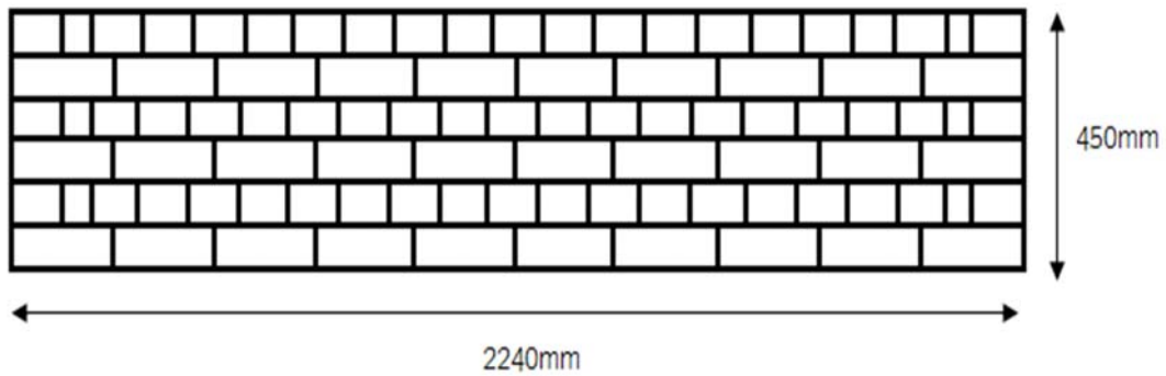
Front elevation
