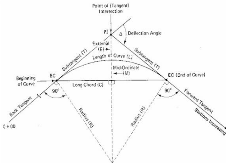
Setting out a horizontal curve
