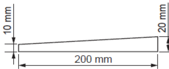
Stair wedge
