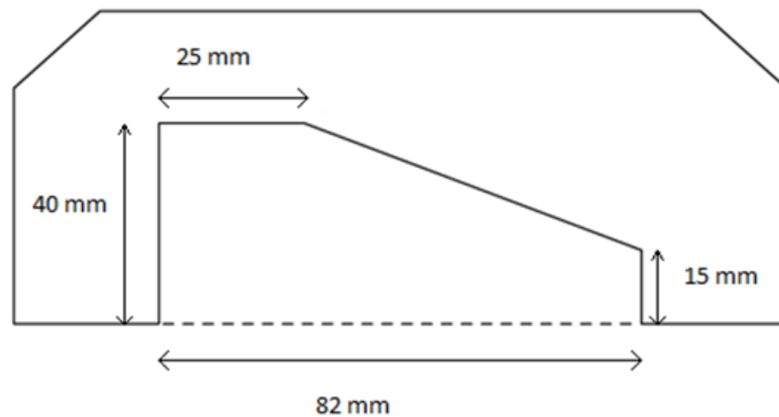
Figure 2 Zinc template for architrave
