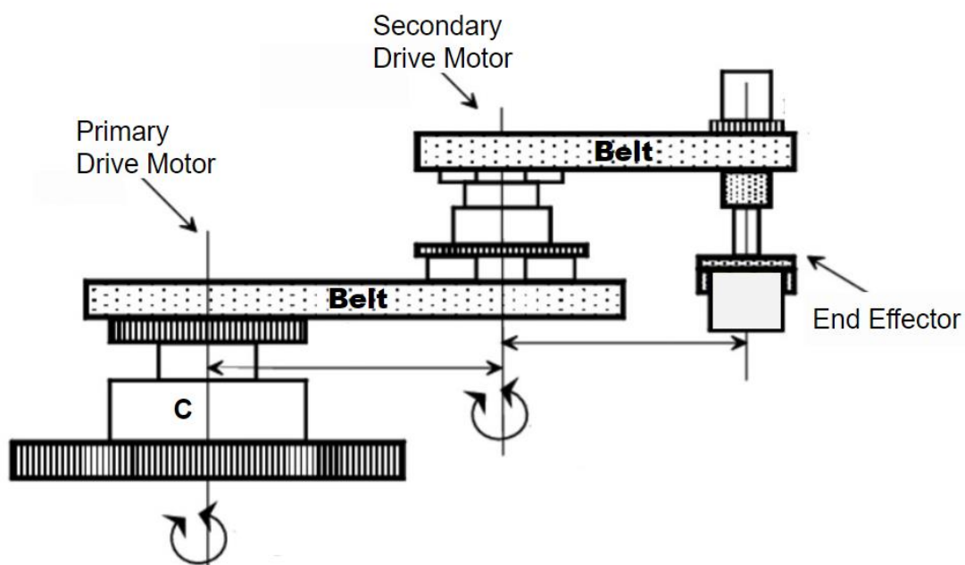
Figure 2 – System schematic
