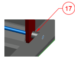
SCISSOR LEG / BRACKET CONNECTION DETAIL 2
