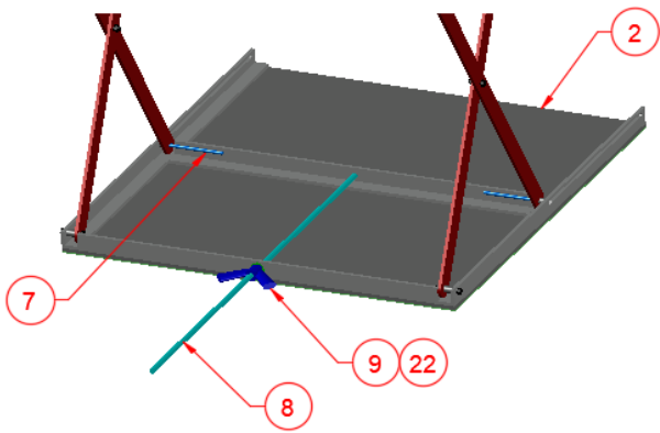
FRONT UNDERSIDE VIEW OF TOP PLATE
