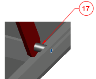
SCISSOR LEG / BRACKET CONNECTION DETAIL 1
