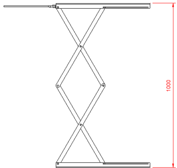
OPEN POSITION HEIGHT INCLUDES NYLON MAT
